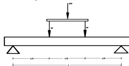
Figure No. 2. Typical Two Point Loading Arrangement
