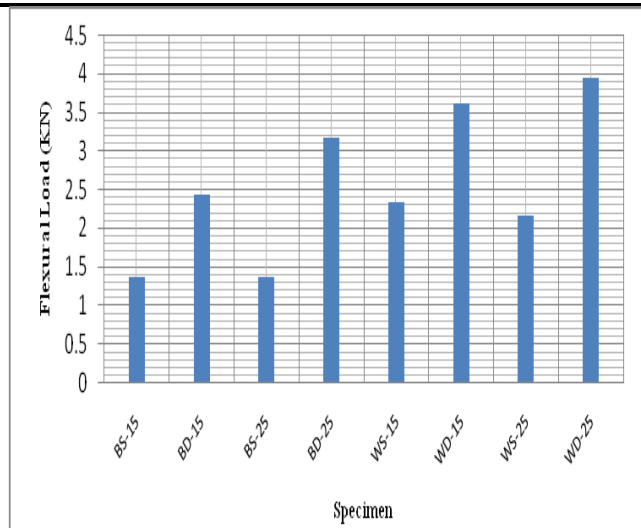
Graph No.2.28 Days Curing Flexural Load Carrying Capacity
