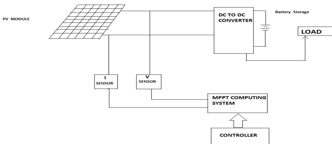
Fig.5. Schematic of diagram MPPT system.
