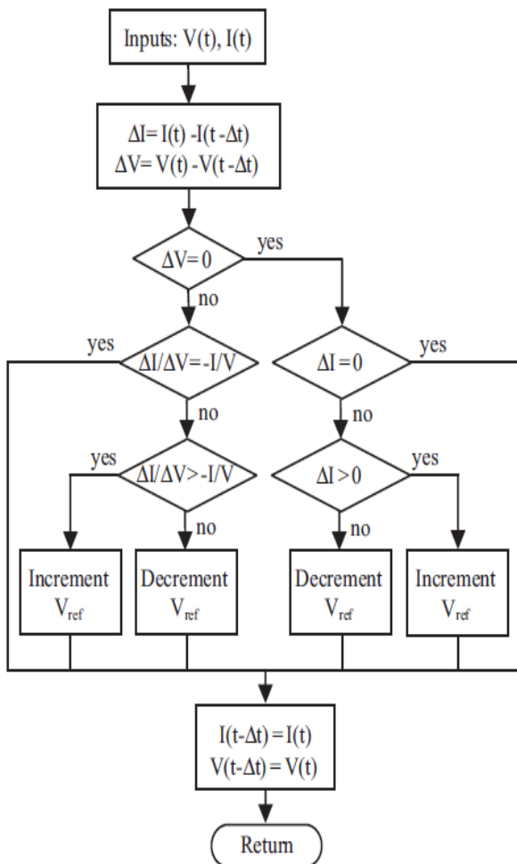
Fig.2. Incremental Conduction algorithm
