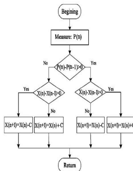
Fig.1. Perturb & Observe algorithm
