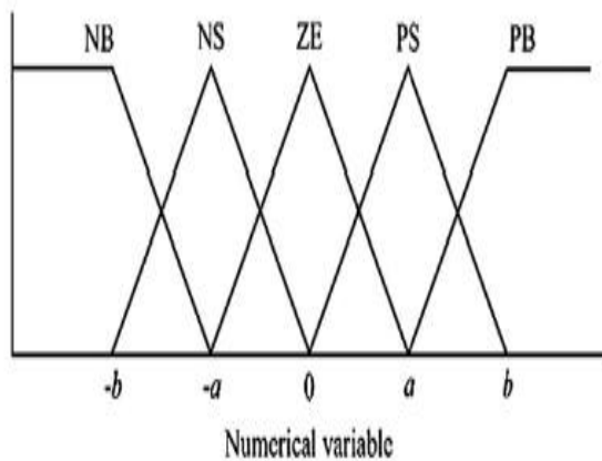
Fig4. Membership function for inputs and output of fuzzy logic controller
